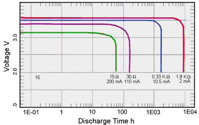
Continuous discharges at 25°C
